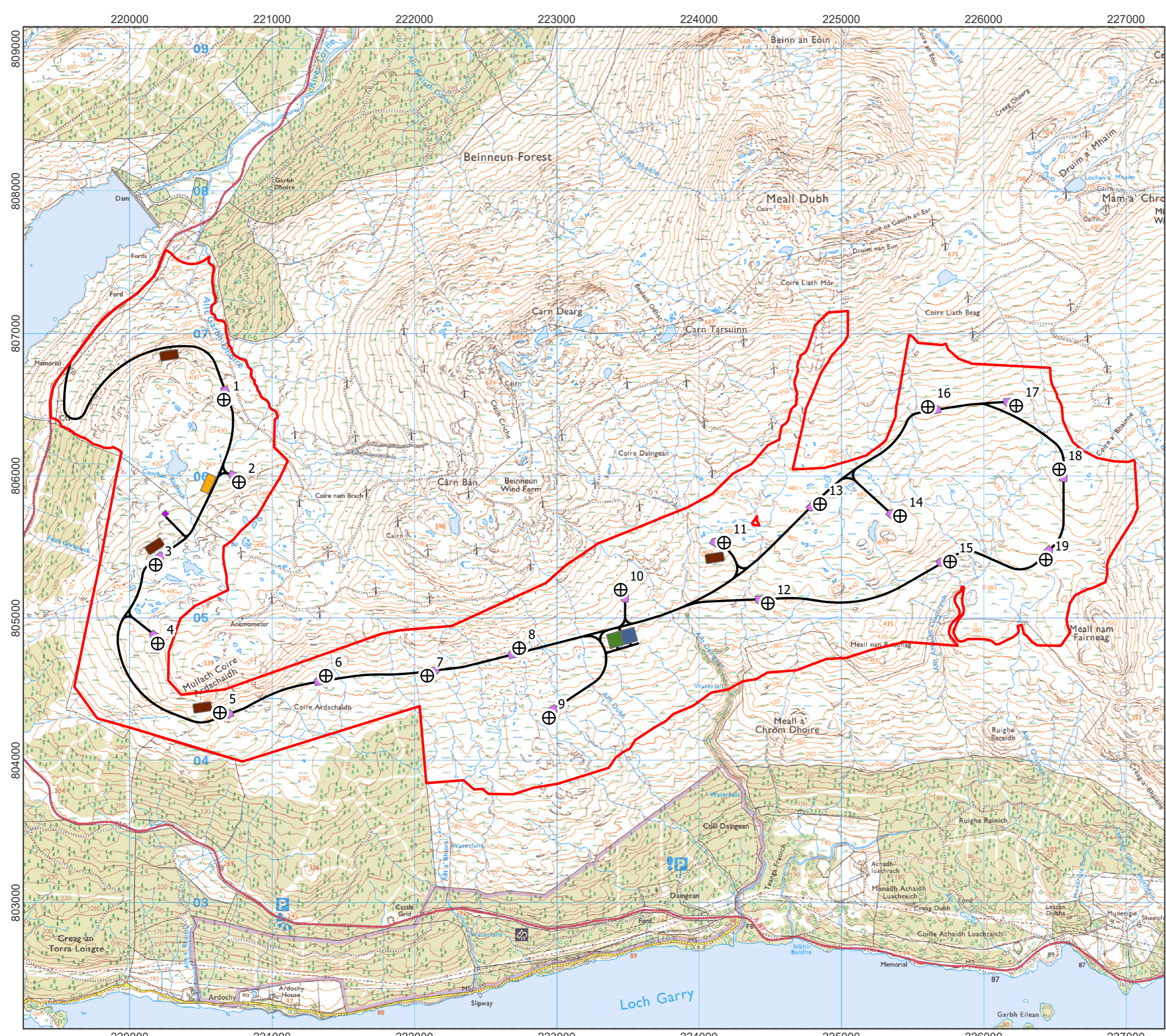
Figure 3.3d: Final Design
